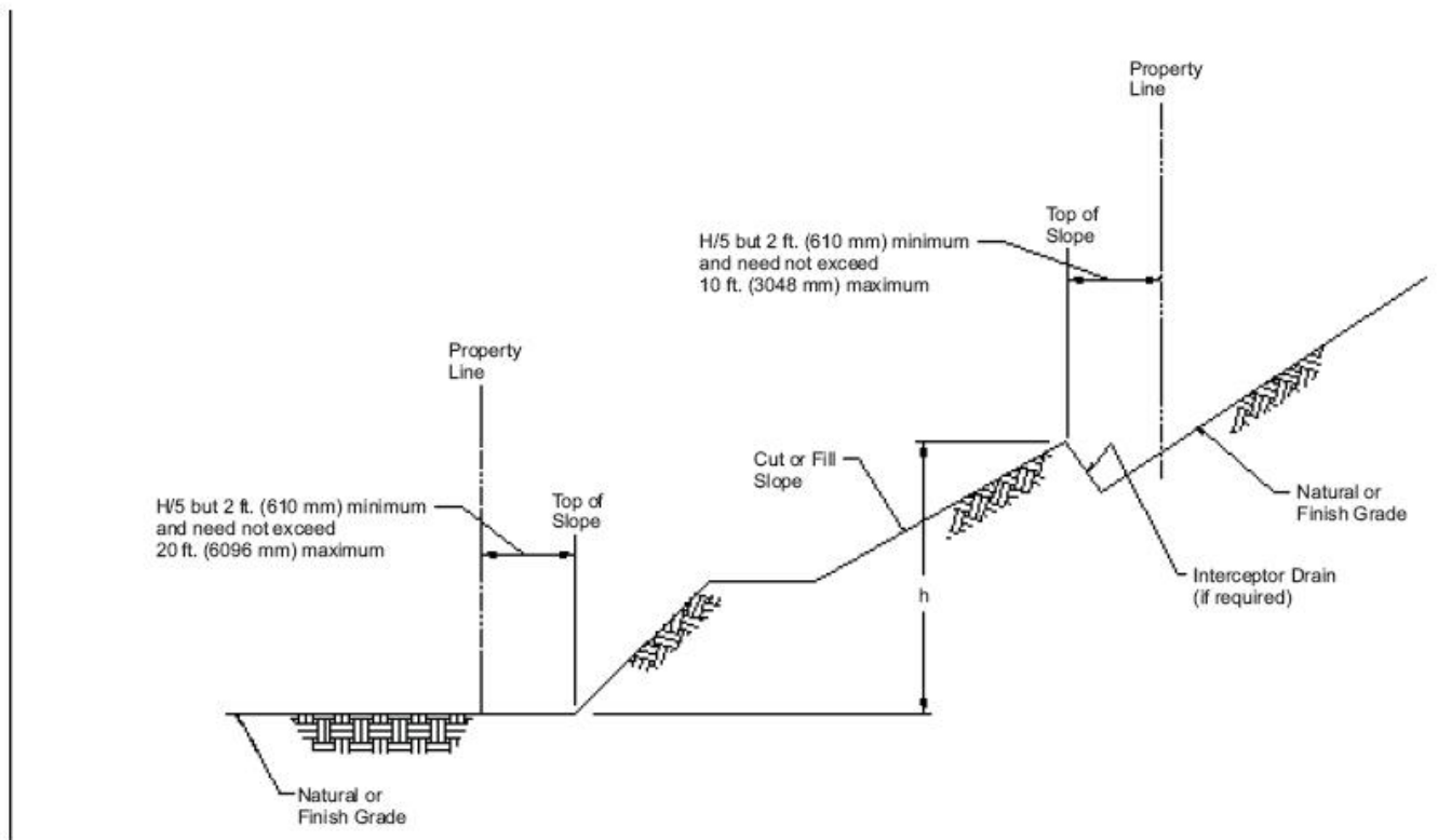
FIGURE J108.1 DRAINAGE DIMENSIONS
