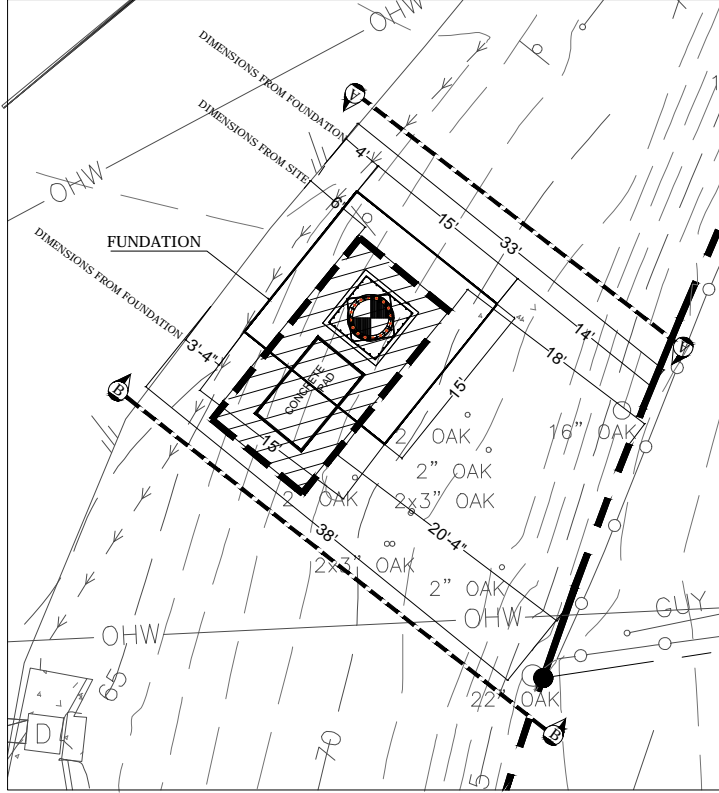
SITE PLAN SODA CANYON
