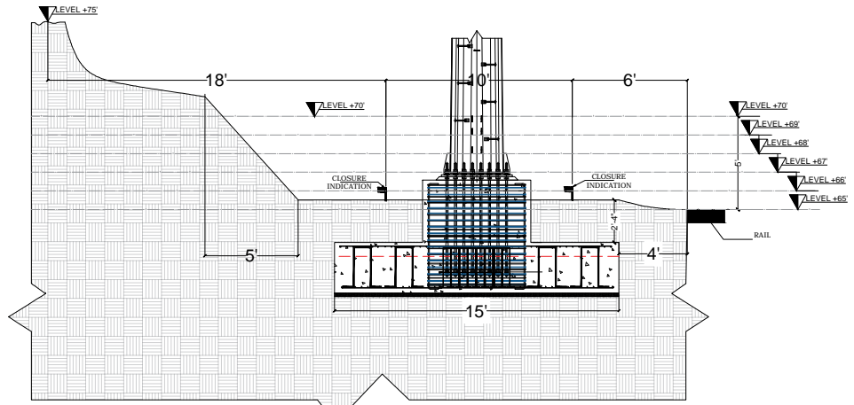
VIEW A-A SODA CANYON
